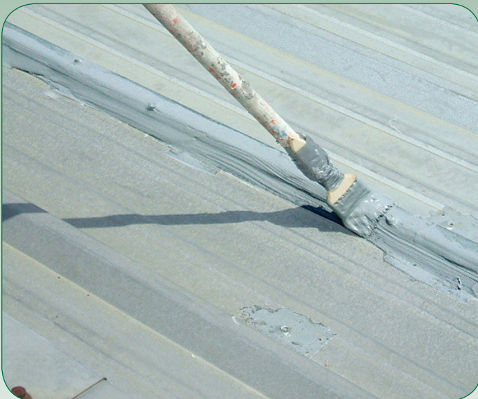
HER POLYURETHANE SEALANT is applied to the seams, fasteners and penetrations and then smoothed with a brush.
